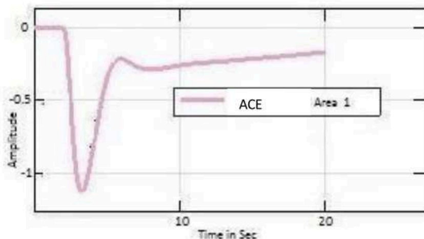
Figure8:Area1Areacontrolerror
