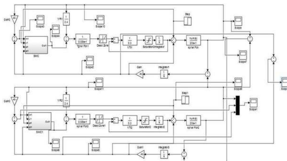
Figure5:Simulinkmodelfortwo-areainterconnectedpowersystem
