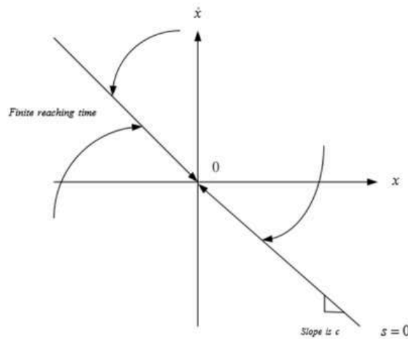
Figure 4: Sliding Surface
