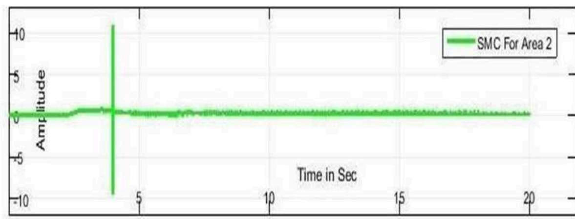
Figure11:area2Controlsignalu2in
