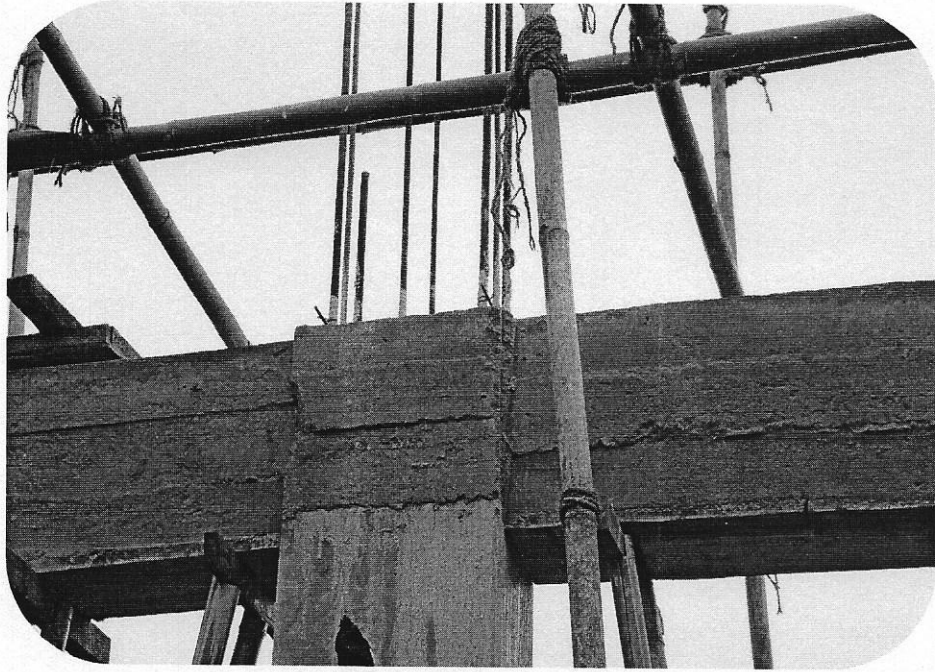
View of reinforcement
