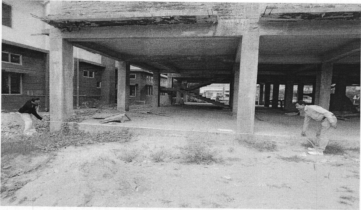
Measurement taking of the total plinth area of the ( G+2) building for Seminar Hall, Computer Centre and facilities for Car parking at Darrang College, Tezpur, Assam
