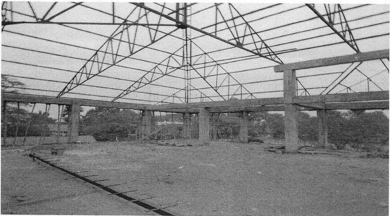
View of Struss work in the (G+2) building for Seminar Hall, Computer Centre and facilities for Car parking at Darrang College, Tezpur, Assam
