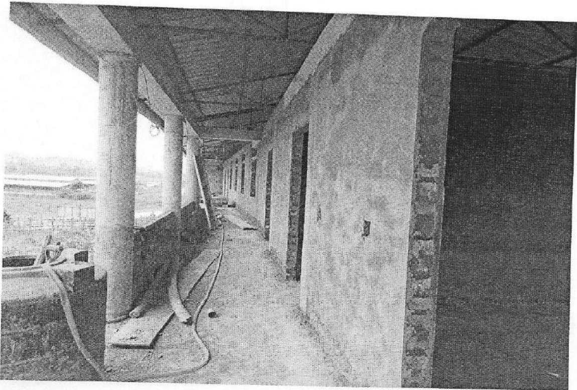
View of the 1 st floor of the Girl hostel
