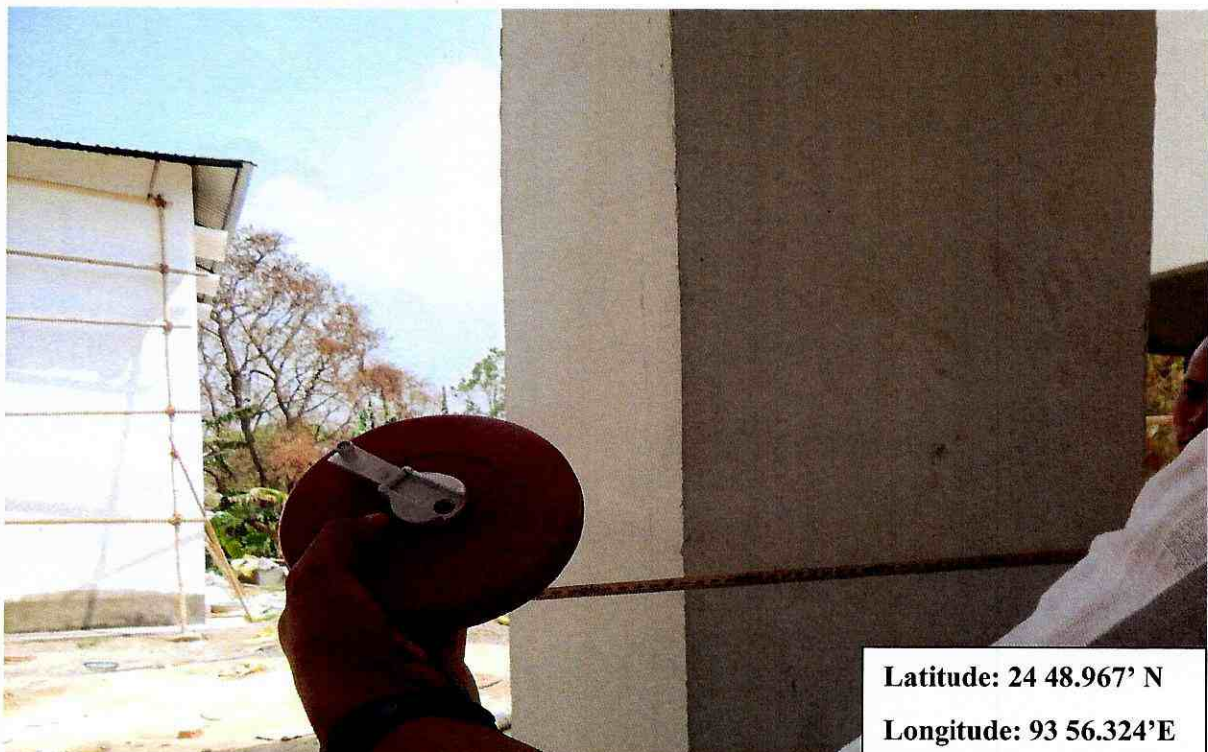
Photo of the inspection team measuring the column of the building for the “Construction of Boys hostel (RCC+G2) with Toilets at Jawaharlal Nehru”, Manipur.
