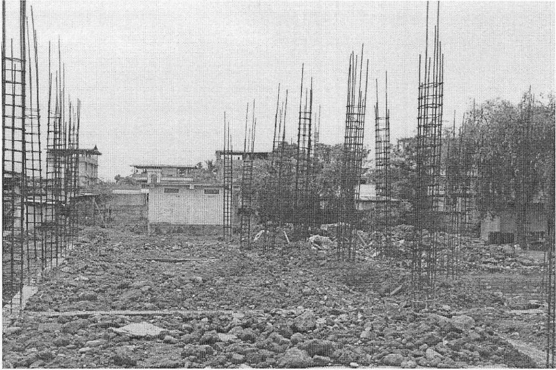
Photo showing the columns erected for Hostel
