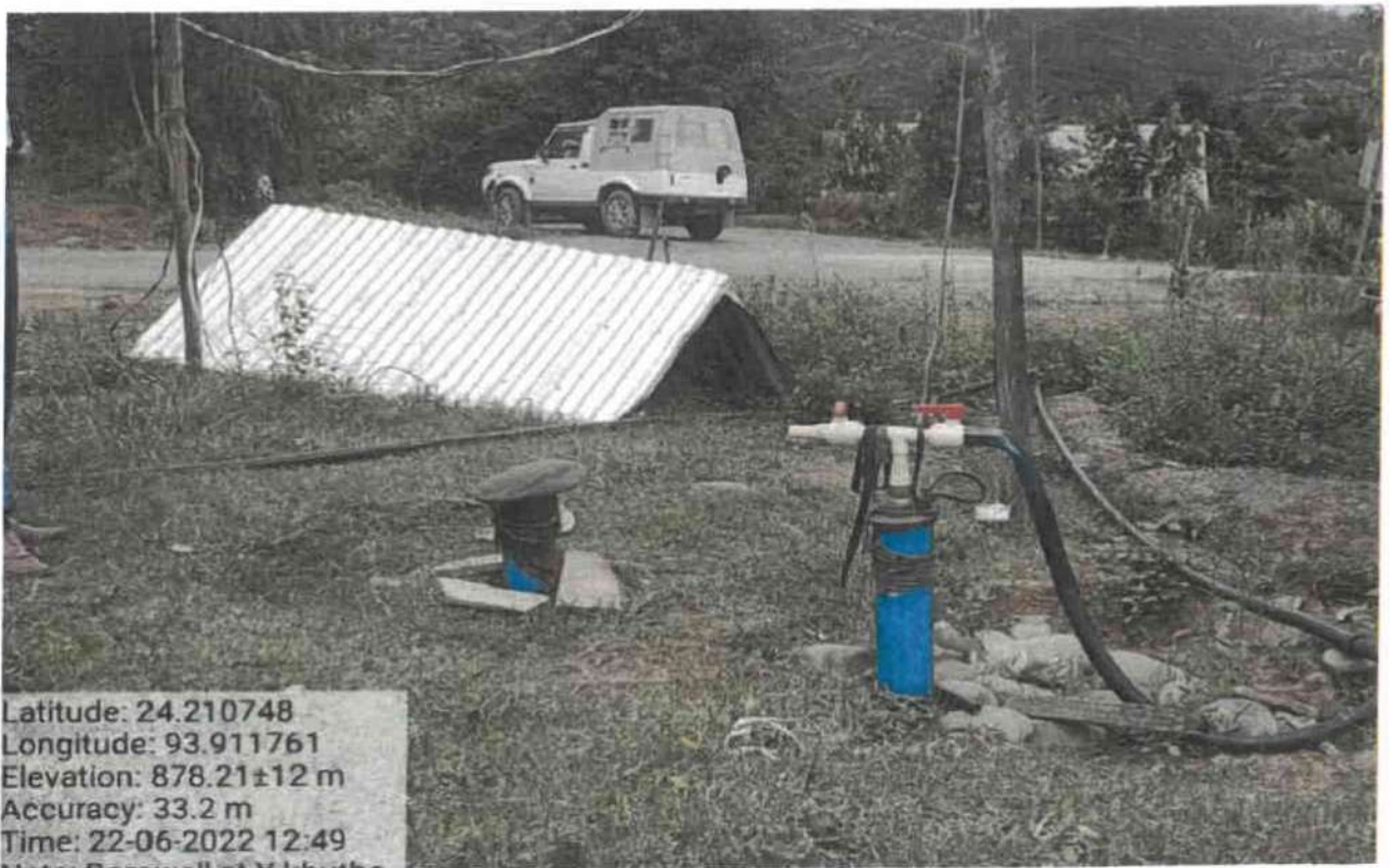
Photo of the “Installation of borewell at Y. Khutha Village” – Location 3
