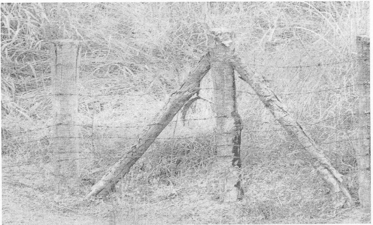
View of fencing with locally available material at Hija village
