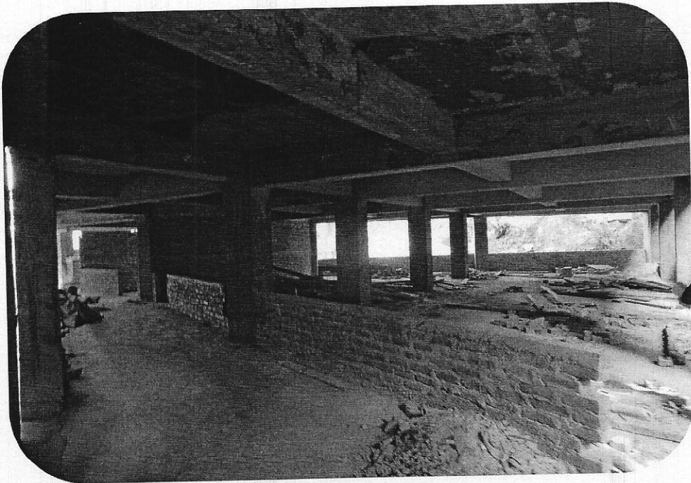
View of Top floor
