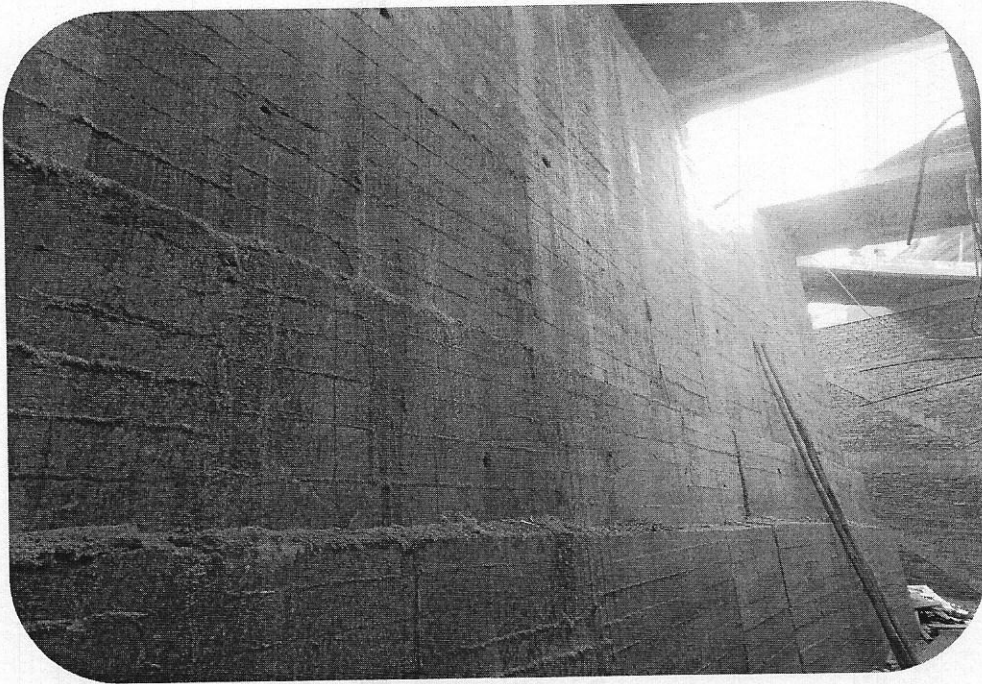
View of 6m height RCC retaining wall
